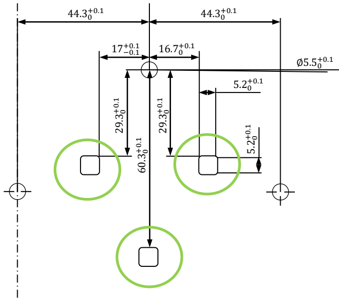
Hole patterns for the upfitter bracket: Measurement and tolerances in millimeters
