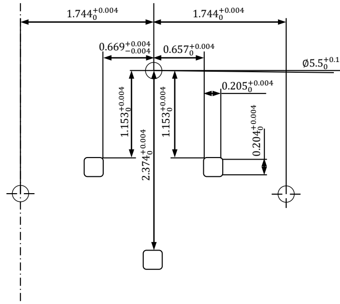
Hole patterns for the upfitter bracket: Measurement and tolerances in inches
