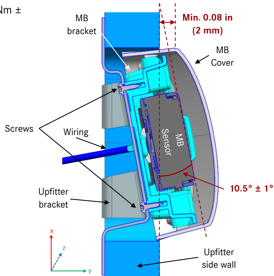
Horizontal Cut (Top View)
